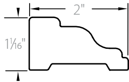
Rake Mould
